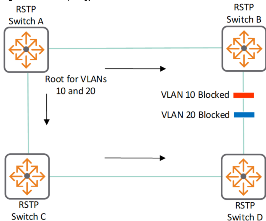
Figure 1 RSTP topology with VLANs 10 and 20 blocked
